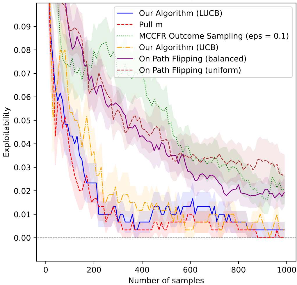
Kuhn Poker, Player o
